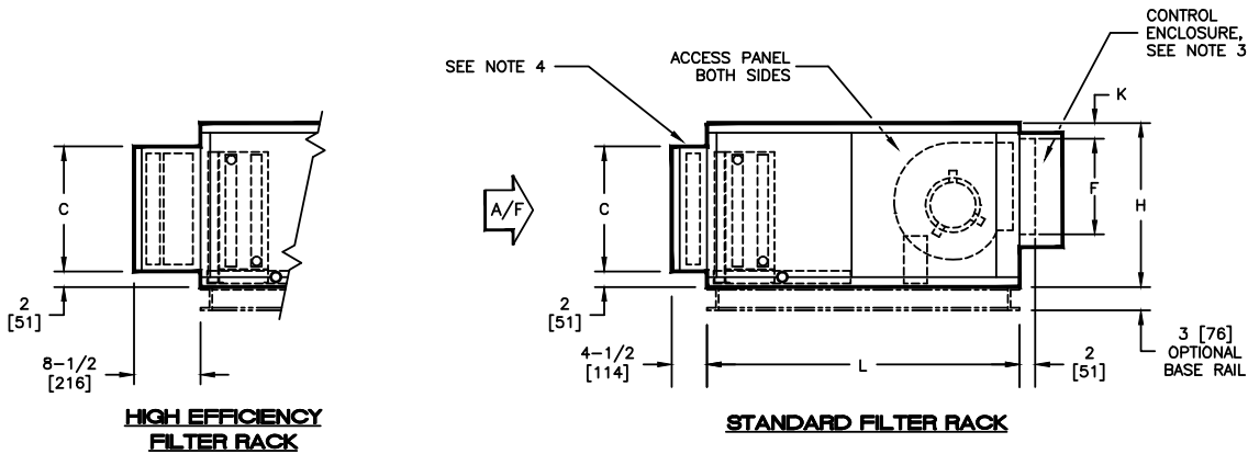
SIDE VIEWS
