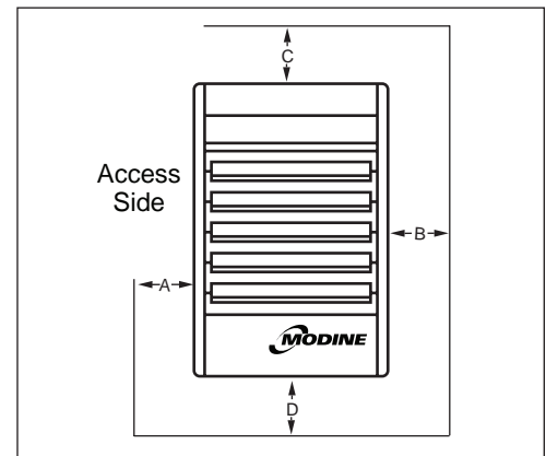
Figure 20.2 - Combustible Material and Service Clearances
